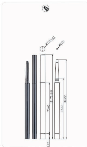
MPA-252 Ø7x121.4mm
