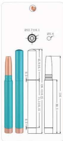
Ø12.7x126.4mm MPA-219
