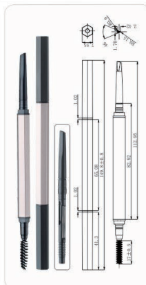
Ø7.5x7.5x149.8mm MPA-165
