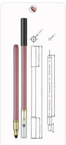
Ø9.3x175mm SP-04
