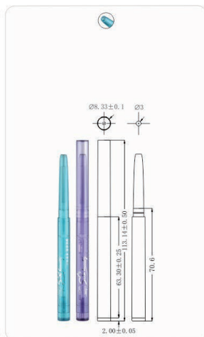
MPA-73 Ø8.3x113.4mm
