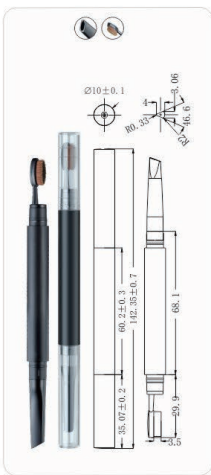
MPA-35 Ø10x142mm
