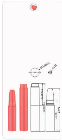
MPA-242 Ø13.1x72mm
