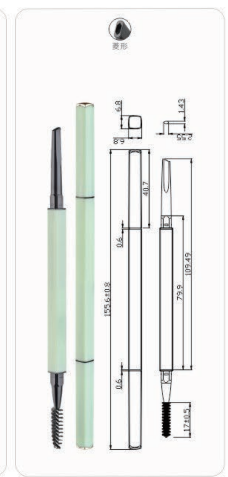
Ø6.8x6.8x155.6mm MPA-230
