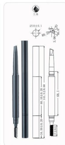
MPA-76 Ø10x142mm
