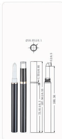
MPA-101 Ø10.03x107.6mm
