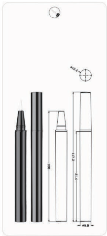
Ø10.4x117mm EYE-01
