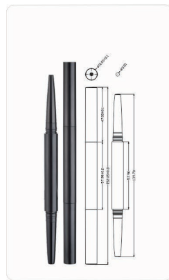
MPA-255 Ø8.5x154.1mm
