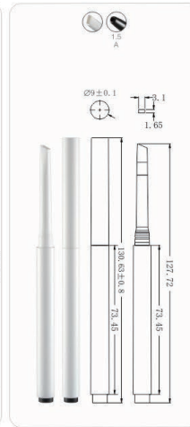
MPA-88 Ø9x131.2mm
