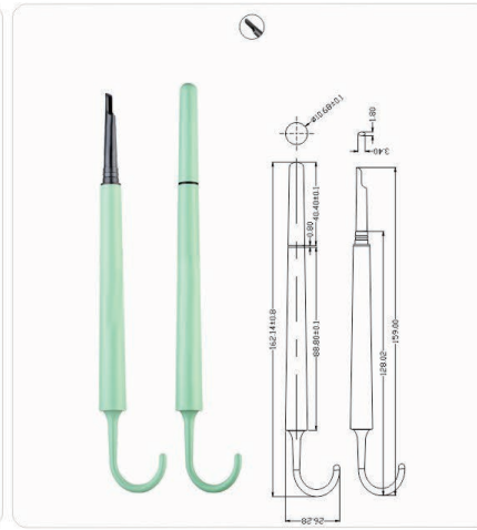
MPA-243A Ø10.65x164mm ZL202230538131.0
