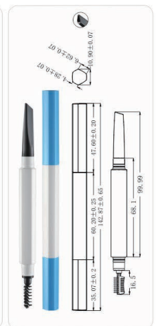
MPA-80 Ø10x142.8mm
