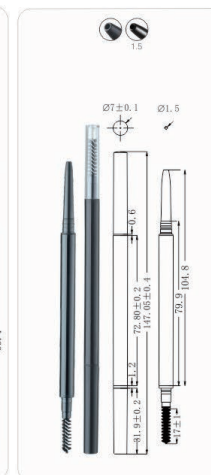
MPA-116 Ø6.8x146.1mm
