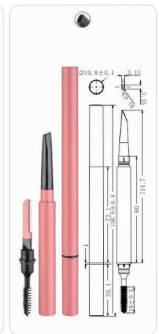
Ø10.8x158.75mm MPA-205
