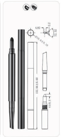
MPA-26C Ø10.8x153mm
