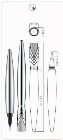
Ø14.4x139.1mm EYE-21
