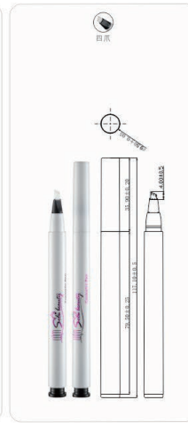
Ø9.6x118.55mm EYE-29
