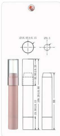
MPA-100 Ø18.05x109.3mm
