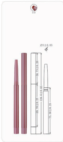
MPA-01 Ø8x121/132mm
