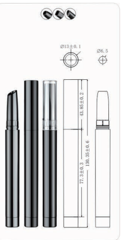
MPA-05 Ø12.8x130mm
