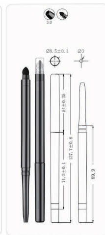
MPA-16 Ø8.5x137mm
