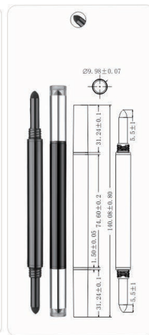
MPA-18 Ø10x139mm
