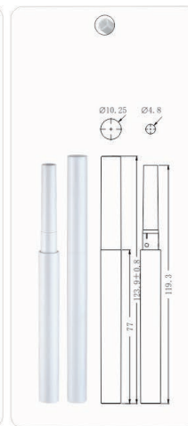
Ø10.25x123.9mm MPA-186
