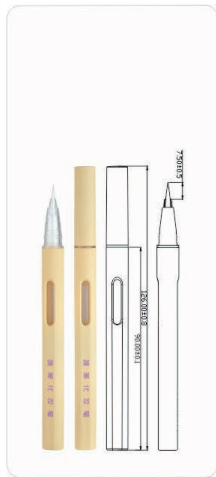
Ø9.8x126mm EYE-80
