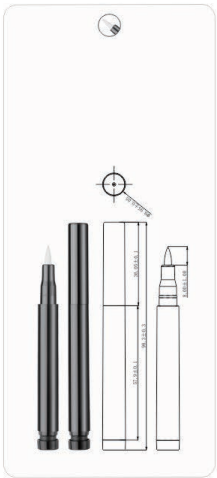
Ø10x101mm EYE-04
