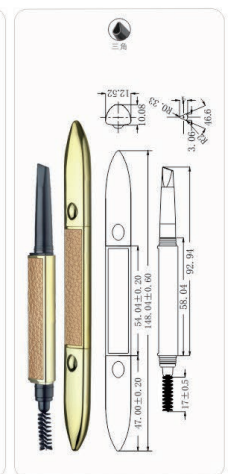
MPA-138 Ø9.8x12.6x147.8mm
