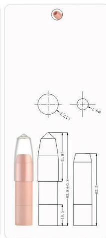
MPA-09B Ø18.2x83mm
