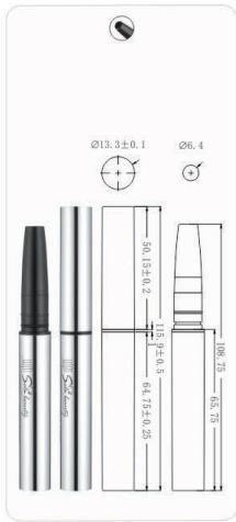
MPA-81 Ø13.3x115.9mm
