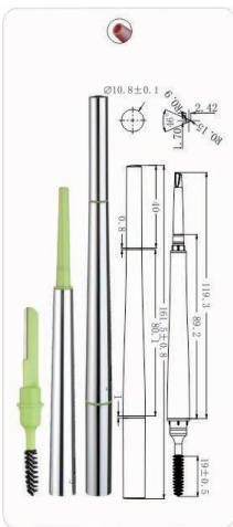
Ø10.8x7x161.5mm MPA-207 ZL202230340555.6
