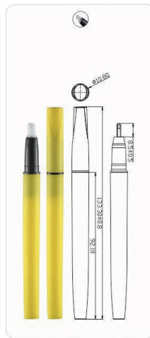
Ø10.8x133.3mm EYE-35
