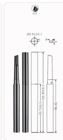
MPA-11 Ø10x122mm
