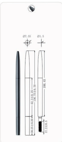
MPA-32 Ø7.4x125mm
