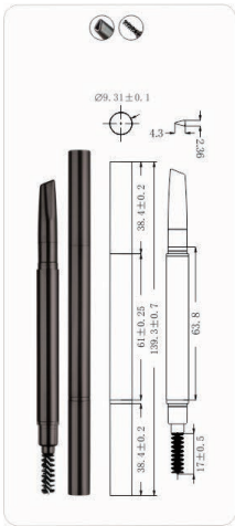
MPA-24 Ø9.3x139mm
