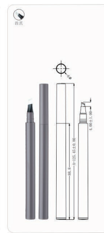
Ø8.5x125.3mm EYE-38B
