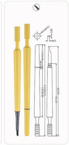
MPA-243B Ø10.65x26.25x164mm
