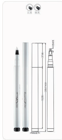
Ø10x135.07mm EYE-27
